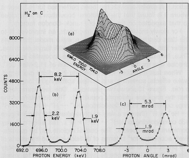
Figure 9. (a) "Ring pattern" and (b, c) "cross" for protons from 1.4-MeV H_2^+ dissociating in an 88-Å-thick carbon foil. 2
