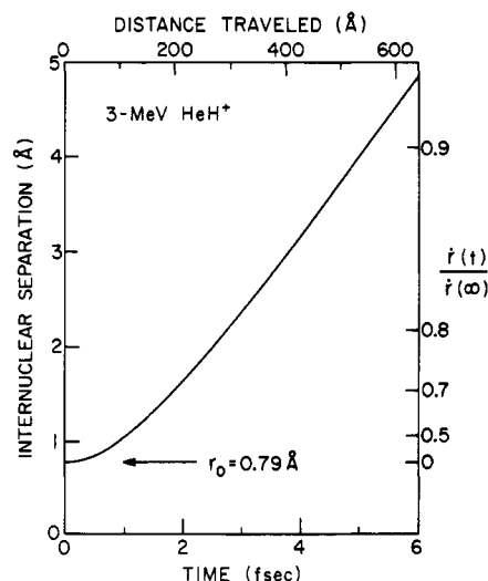
Figure 2. The dependence upon time of the internuclear separation between the \alpha particle and the proton of a \text{HeH}^+ ion whose internuclear separation at t = 0 is 0.79 Å. The right-hand ordinate gives the fractional growth of the Coulomb-explosion velocity as a function of time. The scale at the top shows the distance traveled in the LAB frame by the projectile assuming the beam energy to be 3 MeV.
