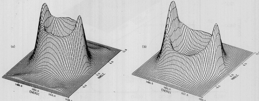
Figure 11. "Ring patterns" for (a) N^+ and (b) N_4^+ fragments arising from the dissociation of 3-MeV N_2^+ in a 75-Å-thick carbon foil. 24
